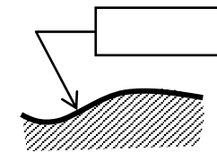
Surface quelconque
